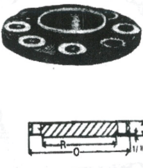
LAP JOINT 1
