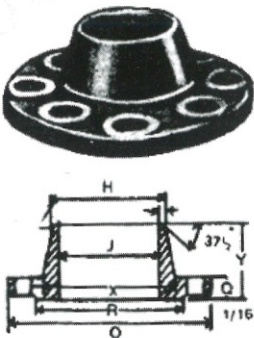
WELDING NECK 1
